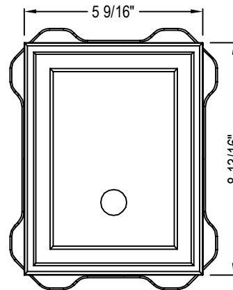
SPLIT BLOCK INSULATE SIDING LOCKING POSITIONS AT 3/4", 1", 1 1/4", 1 5/8"
